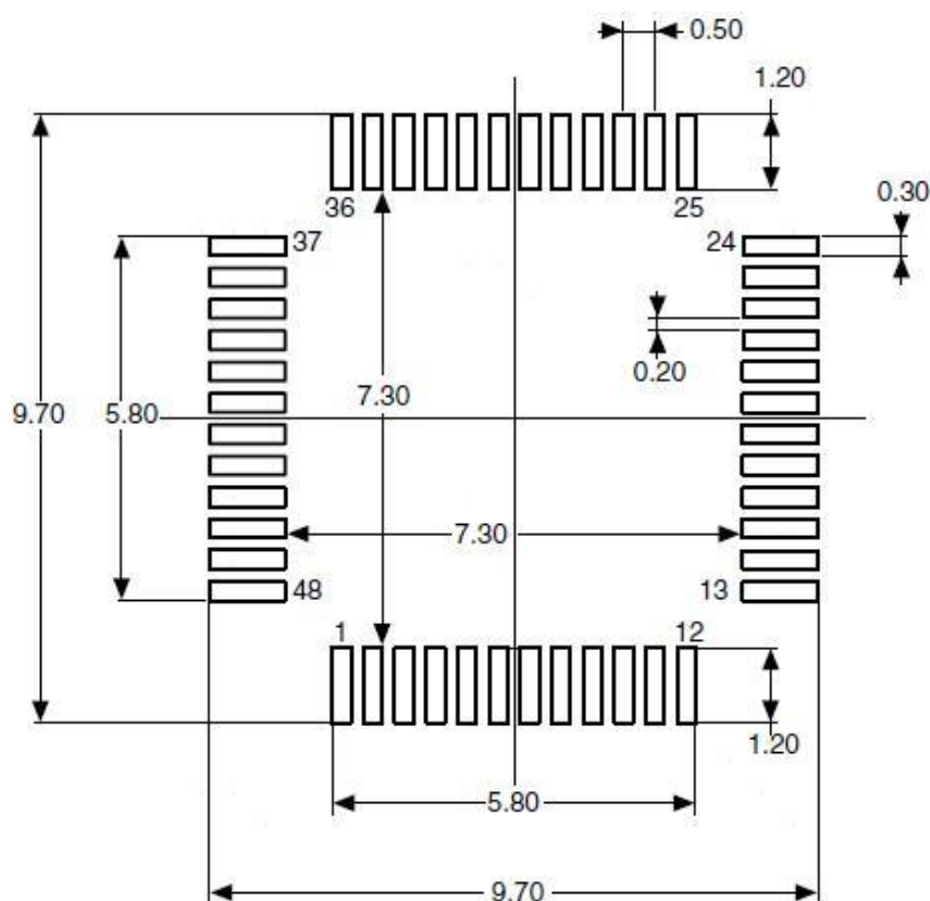
Figure 21 LQFP48, 7×7mm recommended welding Layout
