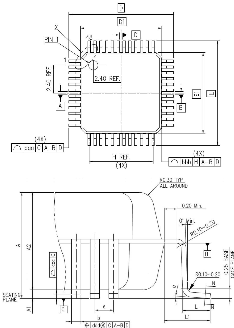
Figure 20 LQFP48 Package Diagram
